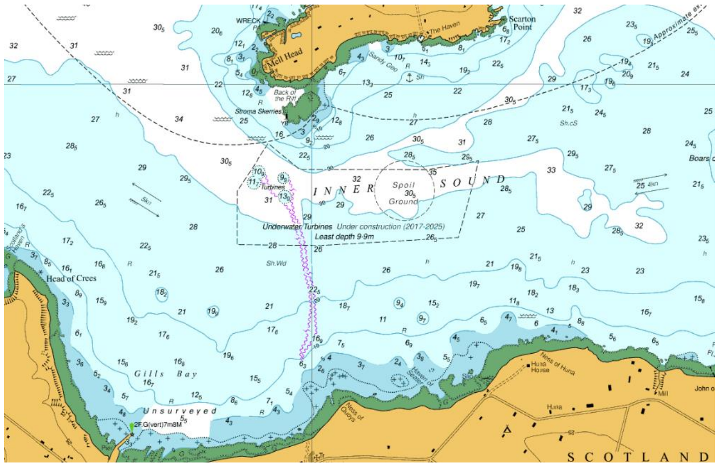
Figure 3 – Chart 2851 © UKHO
