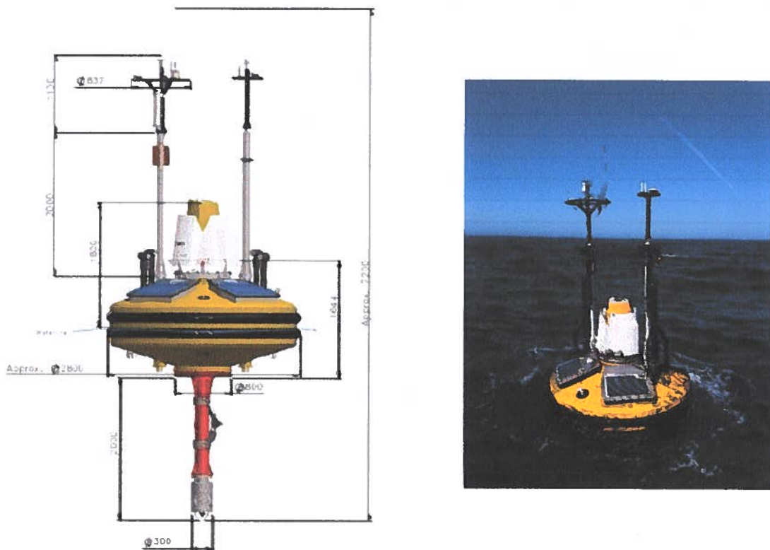
Figure 2: Equipment dimensions (left), example deployment (right)
